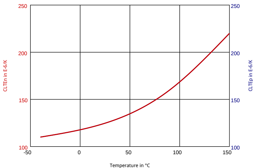
Coeff. of linear thermal expansion, normal (measured on Delrin® 500P NC010)
