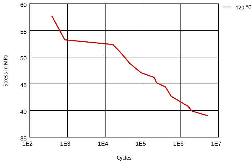
疲劳(Wheller), 拉伸, 10Hz, R=0. mm(干)
